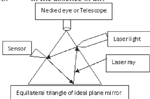
Fig: Experimental Arrangement to Verify Photon is Non-Luminous Particle.
