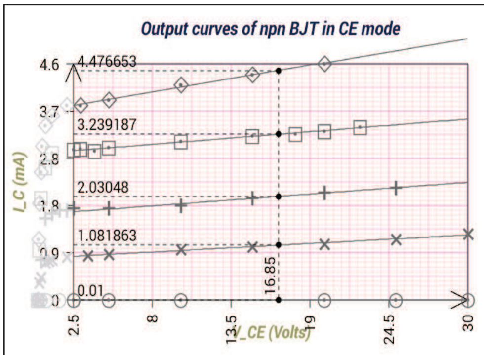
Fig. 3: Example of linear fitting along with Y values obtained at any X value for different data sets.
