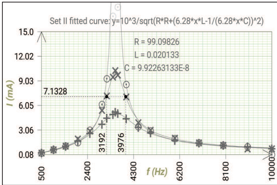
Fig. 4: Example of arbitrary function fitting along with X values obtained at any Y value after fitting
