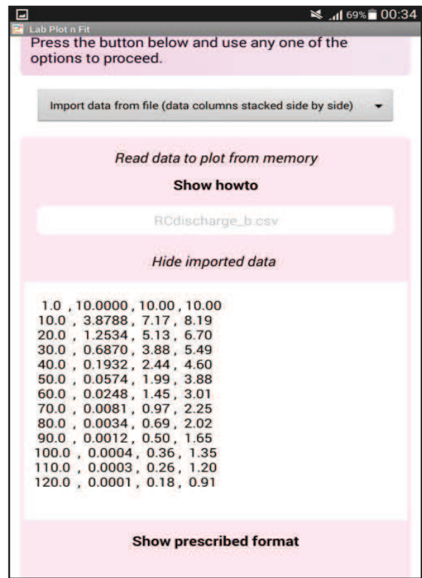
Fig. 2: A screenshot of multi-set data imported from a file
